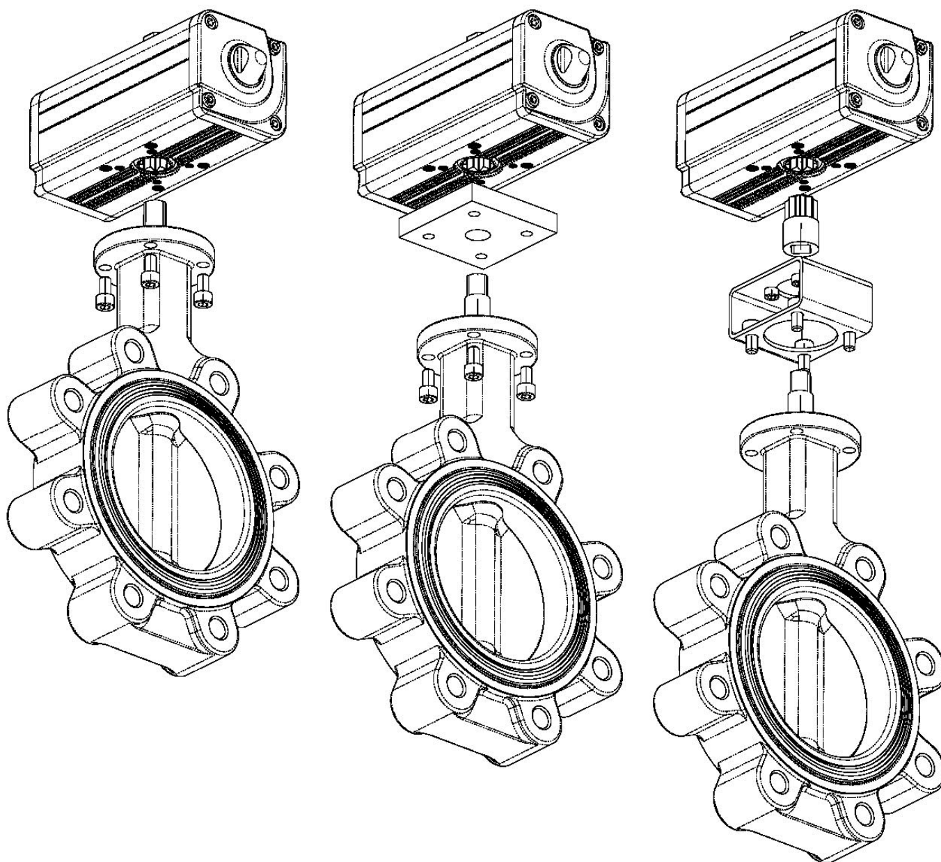
Fig 5,2 – Valve/Actuator assembly: (A) direct-mount (B) plate-mount (C) bracket-mount.
