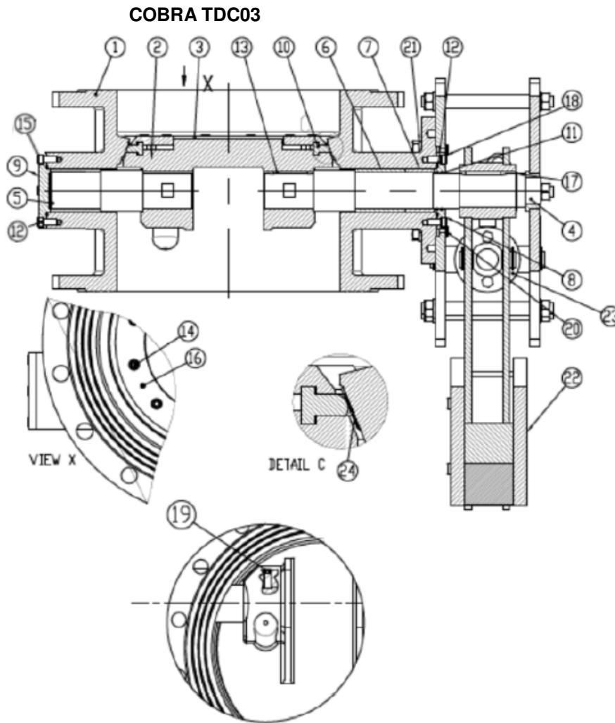
Fig. 4: Exploded view
