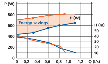
Performance comparison Centrifugal pump – Jet pump
