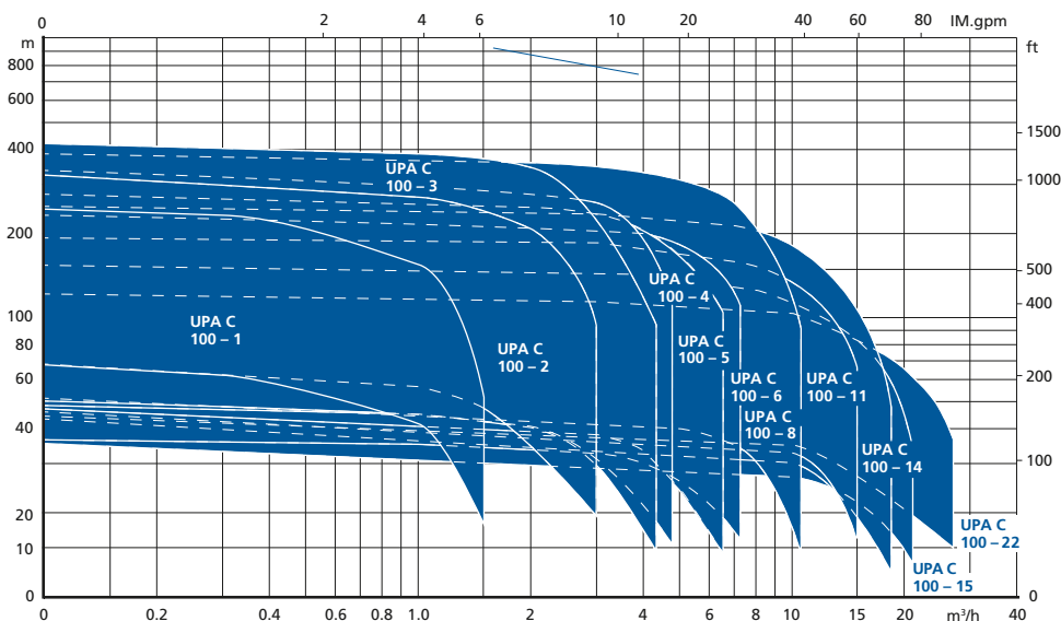
Characteristic curves UPA C 100 CN (60 Hz)
