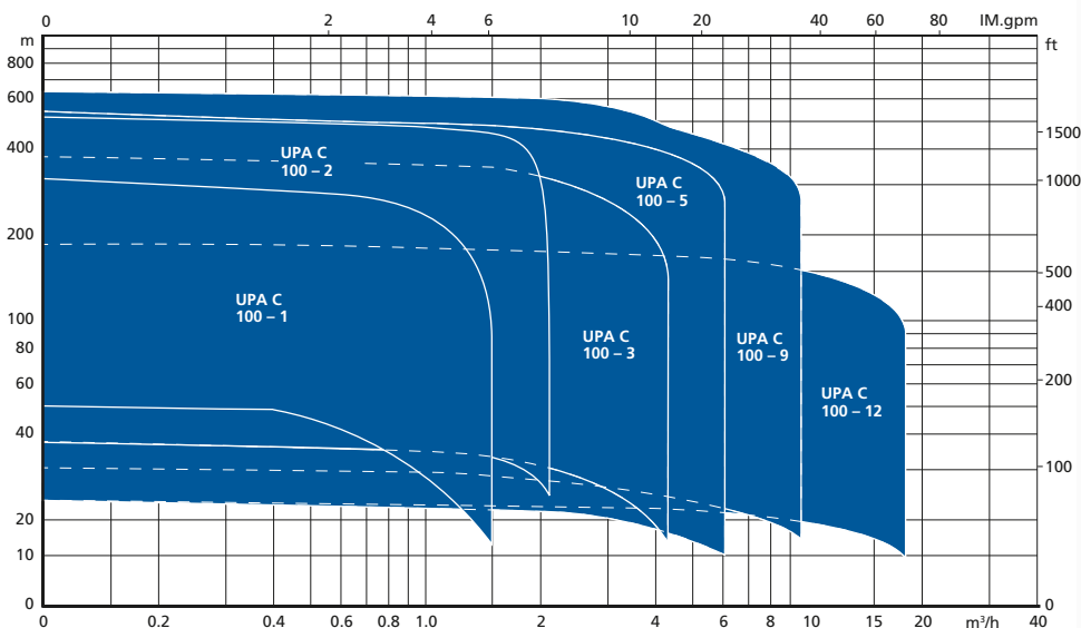
Characteristic curves UPA C 100 CC (50 Hz)
