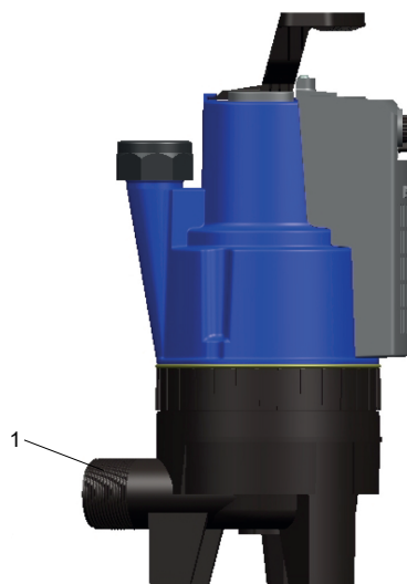
Fig. 11: Connecting the piping, size 354
