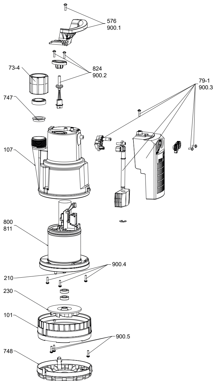
Fig. 28: Exploded view of AmaDrainer 301, 303
