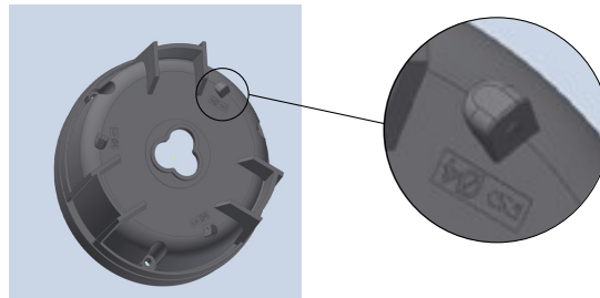
Fig. 4: Cleaning opening
